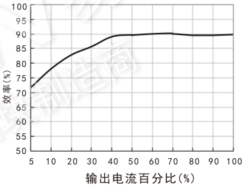
效率Vs输出负载 (V in =24V) URB2405LD-20WR3
