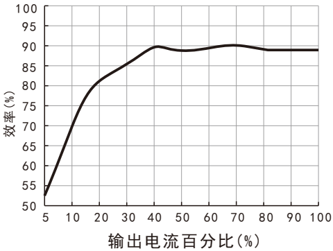
效率Vs输出负载 (V in =24V) URB2405LD-20WR3
