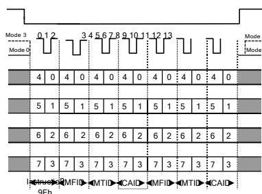
Figure 7.31b Read JEDEC ID(QPI Mode)
