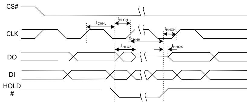
Figure 8.6 Hold Timing
