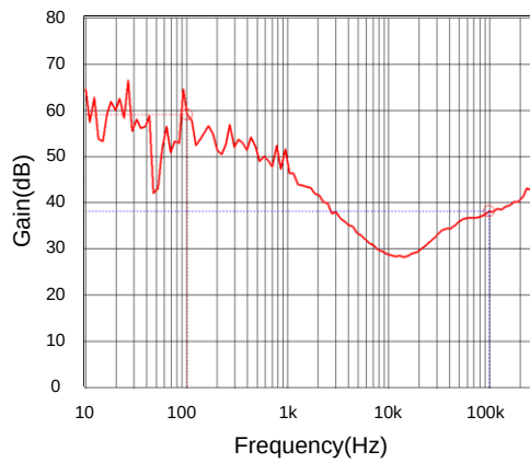
PSRR ( V_{IN}=8V , V_{OUT}=5V , C_{OUT}=4.7\mu F , 10mA Load)
