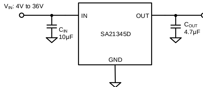
Figure 1 Schematic Diagram
