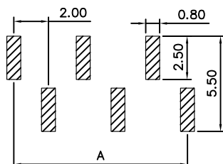
RECOMMEND P.C.B LAYOUT PCB TOLERANCE: ±0.05 (TOP VIEW)
