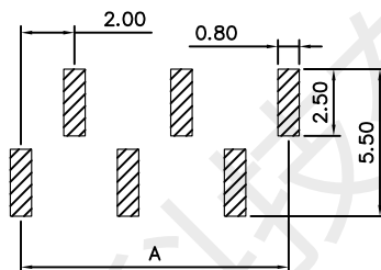
RECOMMEND P. C. B LAYOUT PCB TOLERANCE: ±0.05 (TOP VIEW)
