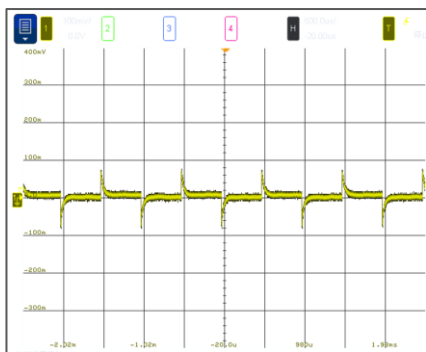
12Vin, 2.5Vout, 2A - 4A, 1A/μs, 跳变频率 1kHz
