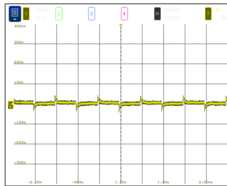
12Vin, 1.2Vout, 2A - 4A, 1A/μs, 跳变频率 1kHz
