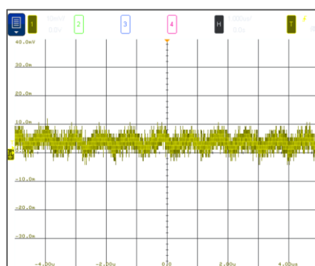
12Vin, 3.3Vout, 负载电流 4A
