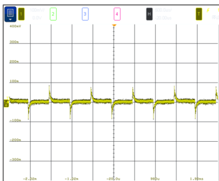
5Vin, 2.5Vout, 2A - 4A, 1A/μs, 跳变频率 1kHz
