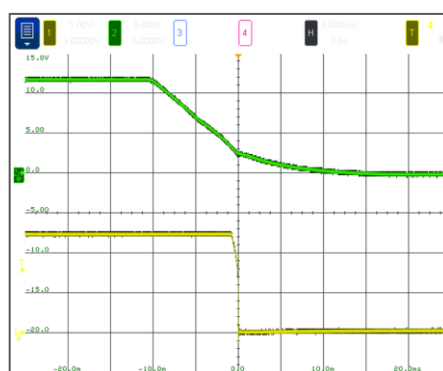
12Vin, 2.5Vout, 4A
