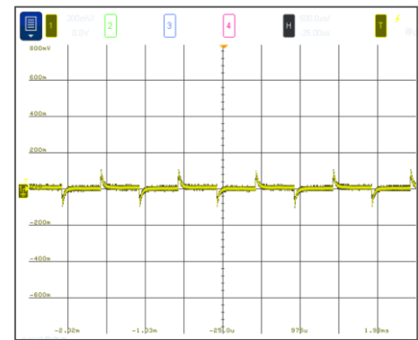
12Vin, 3.3Vout, 2A - 4A, 1A/μs, 跳变频率 1kHz
