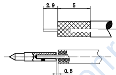
Cable Stripping Dimension
