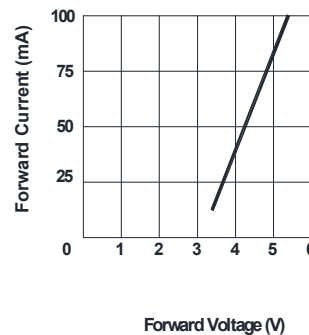
Fig 4. Peak Forward Voltage Vs. Forward Current (100us test pulse, 1% duty cycle)
