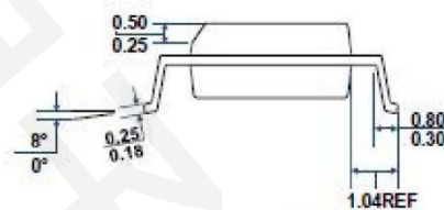
LEFT-SIDE VIEW
