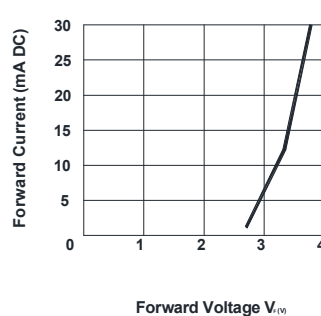
Fig 4. Peak Forward Voltage Vs. Forward Current (100us test pulse, 1% duty cycle)
