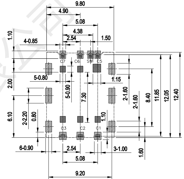
RECOMMENDED P.C.B LAYOUT COMPONENT SIDE (TOLERANCE \pm 0.05 )
