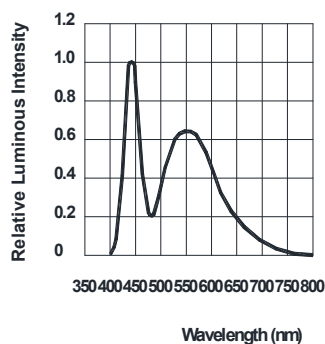
Fig 5. Relative Intensity Vs. Wavelength
