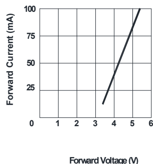
Fig 4. Peak Forward Voltage Vs. Forward Current (100us test pulse, 1% duty cycle)
