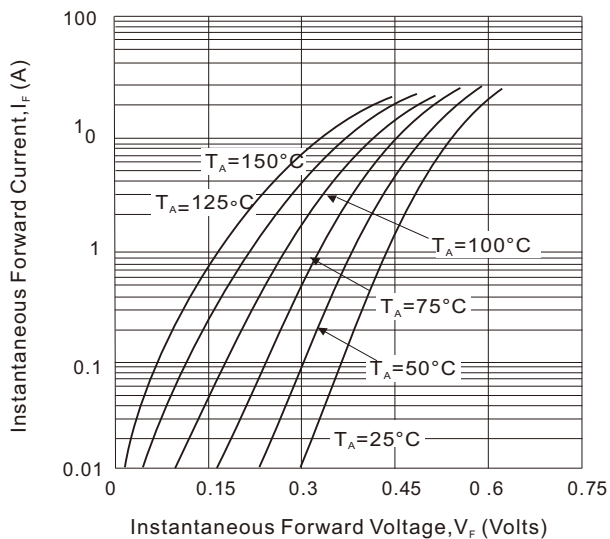
FIG.2-TYPICAL FORWARD CHARACTERISTICS
