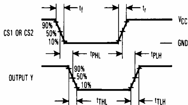
Figure 2. Switching Waveforms
