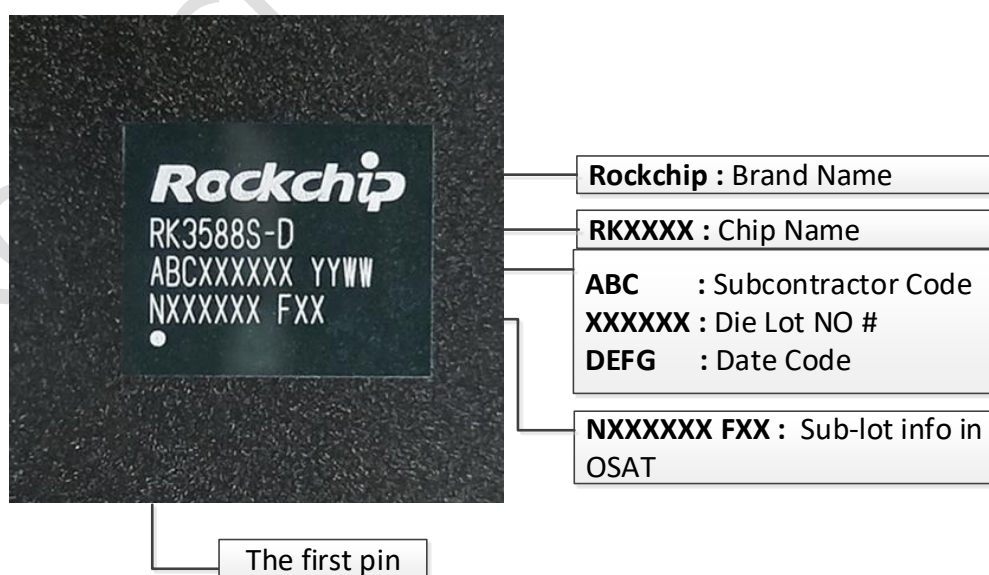
Fig.2-2 Package definition
