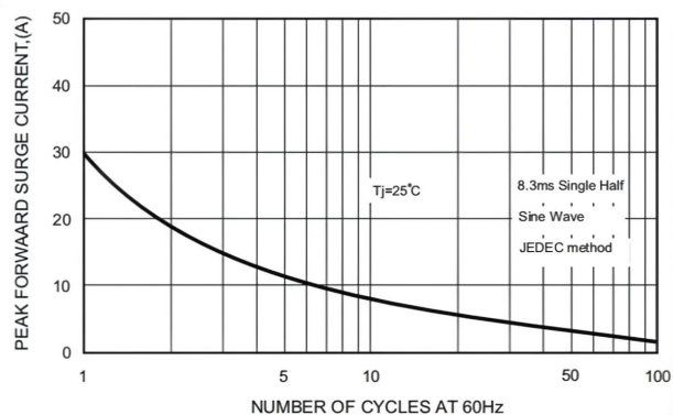
Figure 3: Surge Current Characteristics
