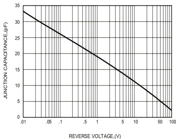
Figure 4: Junction Capacitance
