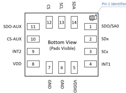
Figure 8. Pins Face Up (Bottom View)
