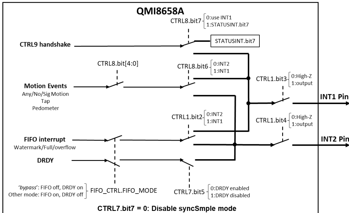
Figure 15. Interrupt Map of Non-SyncSample Mode
