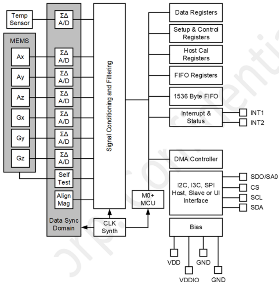
Figure 2. Internal Block Diagram
