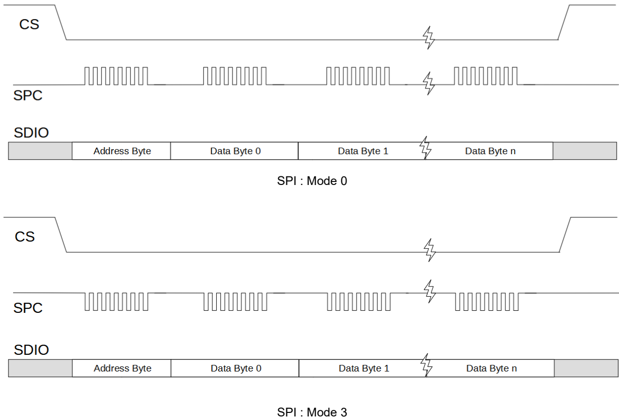
Figure 32. SPI 3-Wire Multi-Byte Read and Write Transactions
