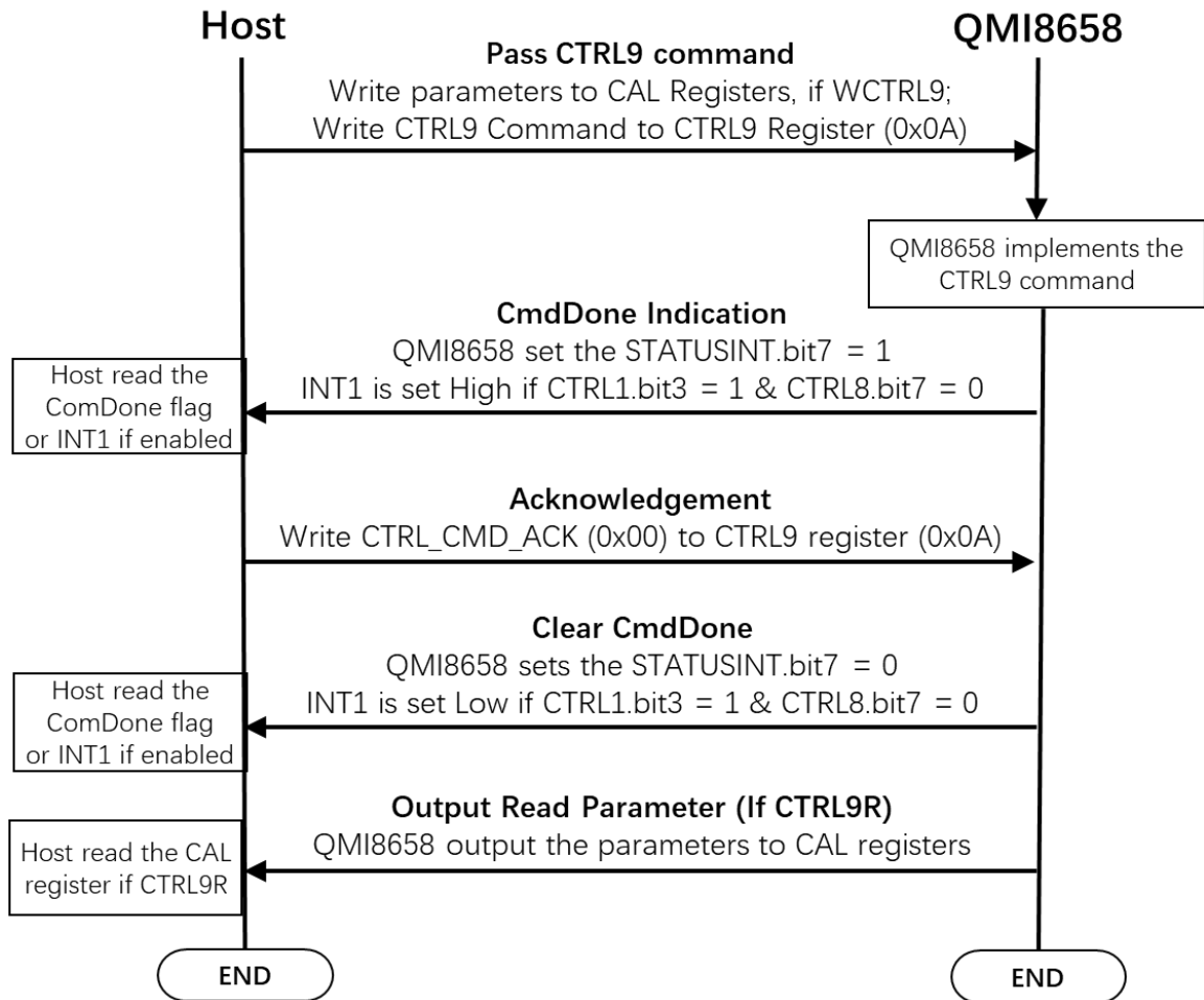
Figure 13. CTRL9 Protocol Flow Chart
