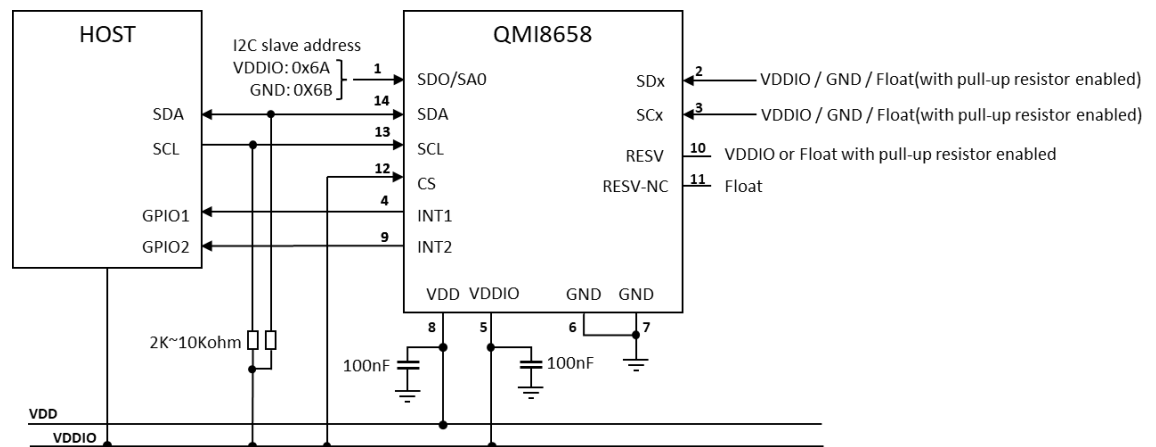
Figure 6. I³C/I²C-UI mode
