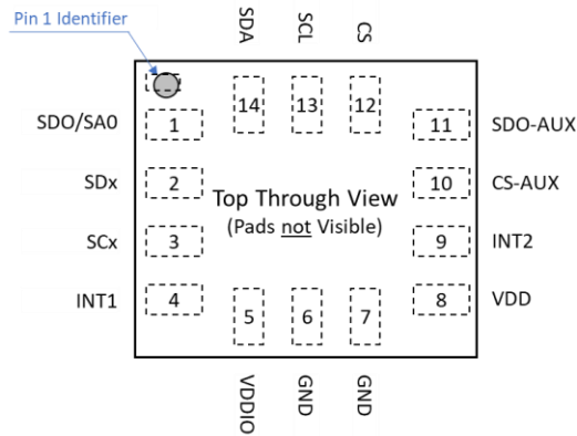
Figure 7. Pins Face Down (Top View)
