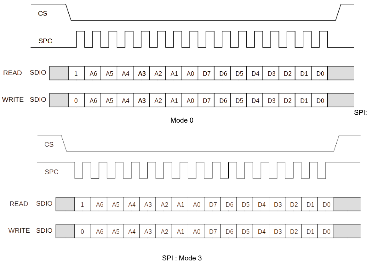
Figure 31. SPI 3-Wire Single Byte Read and Write Transactions
