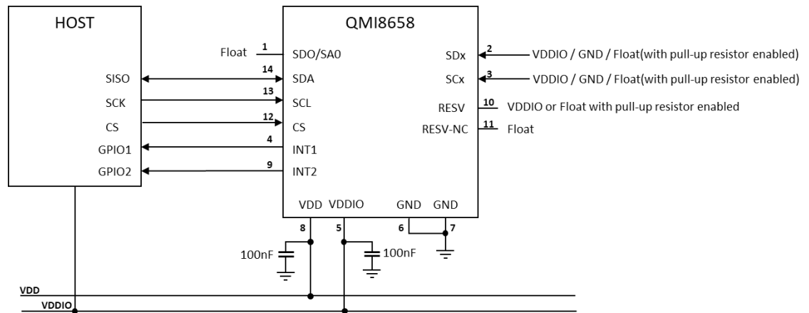
Figure 5. 3-Wire SPI-UI mode
