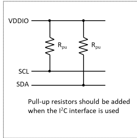
Figure 9. Typical Electrical Connections
