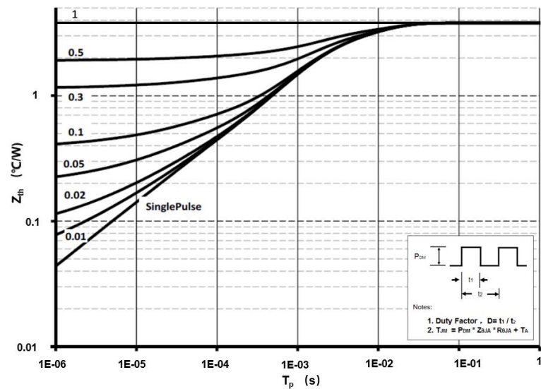
Figure 8. Max. transient thermal impedance
