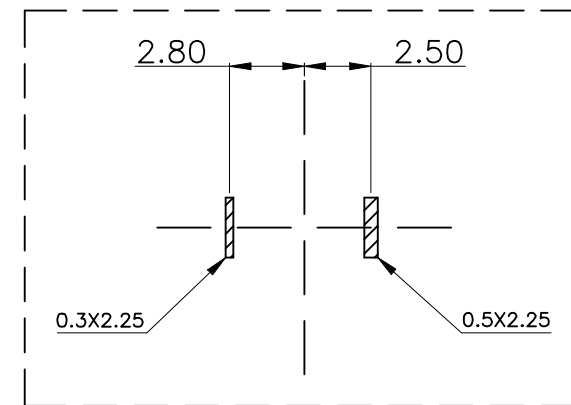
PCB.WELDING DRAWING
