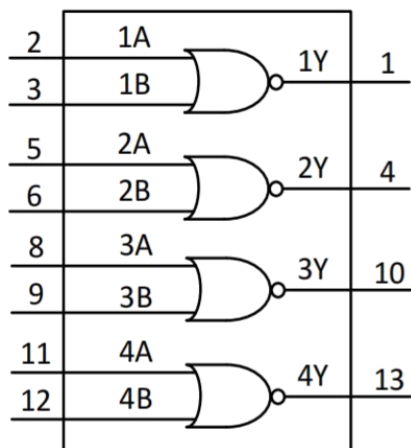
Fig. 1. Logic symbol
