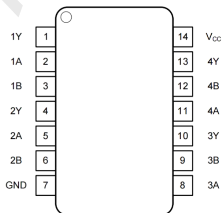
TSSOP-14
