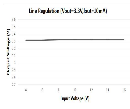
Figure2 . Line Regulation
