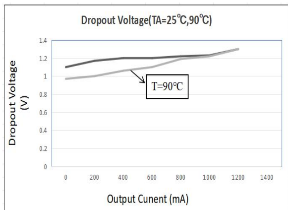
Figure 1. Dropout Voltage
