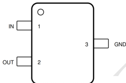
REF31xx SOT23 Package Top View
