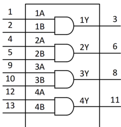
Fig. 1. Logic symbol
