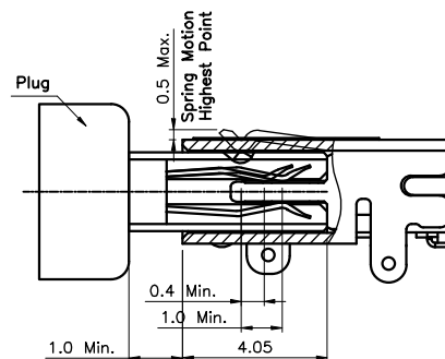
Receptacle and Plug Mated Condition
