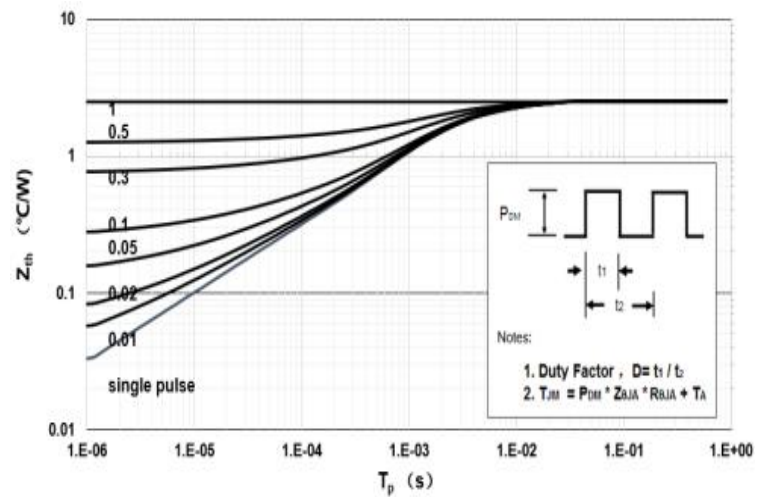
Figure 8. Max. transient thermal impedance
