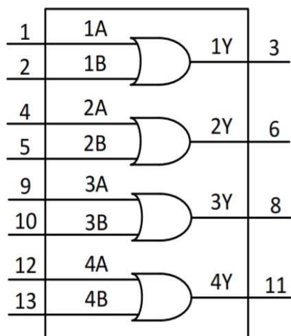
Fig. 1. Logic symbol
