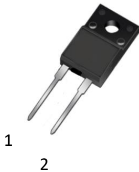
TO-220F-2
