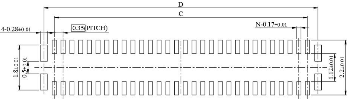
RECOMMENDED METAL DIMENSIONS (THICKNESS: 0.08 mm)
