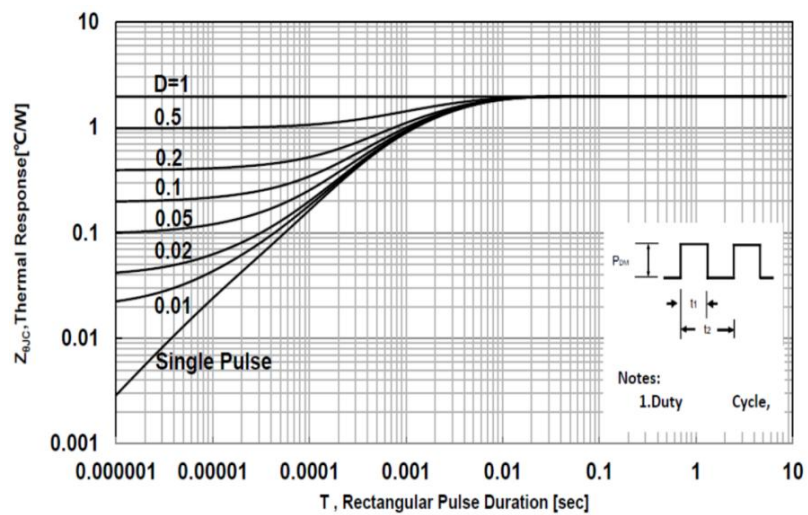
Figure 8. Max. transient thermal impedance
