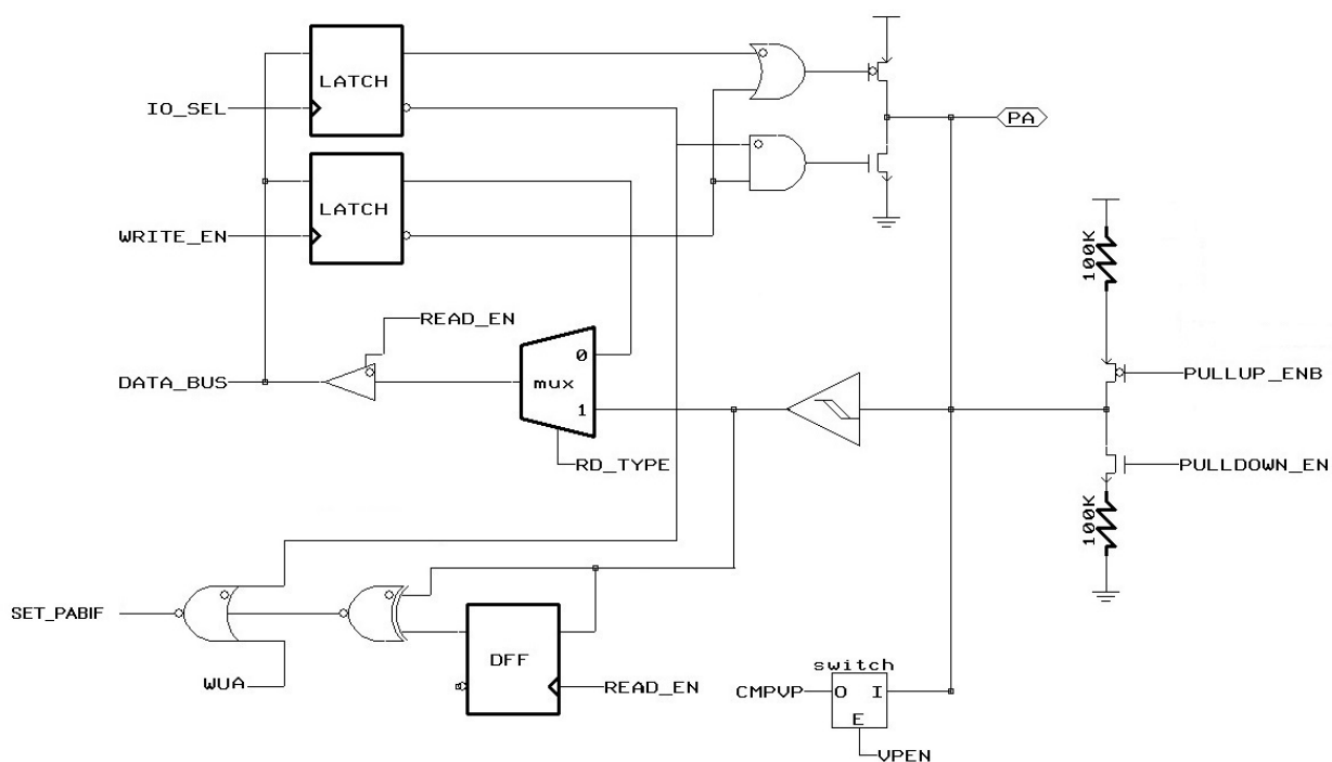
.Figure 5 Block Diagram of PA0, PA1, PA2
