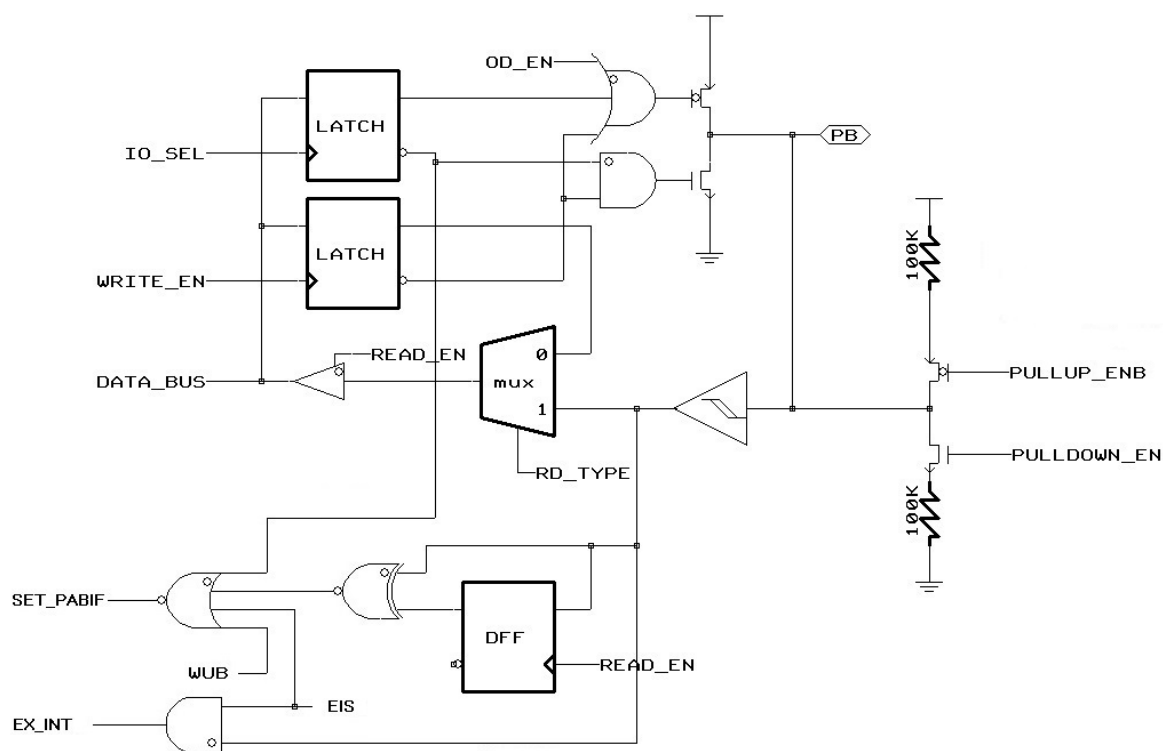
Figure 12 Block Diagram of PB0, PB1
