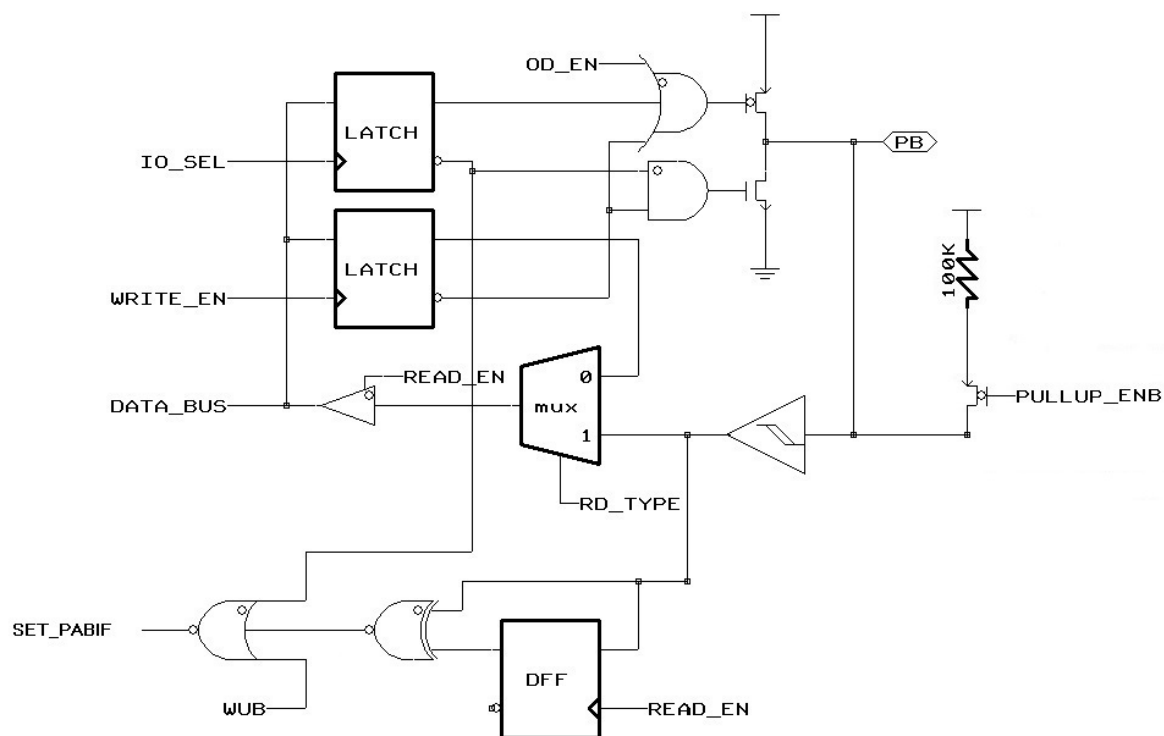
Figure 15 Block Diagram of PB4
