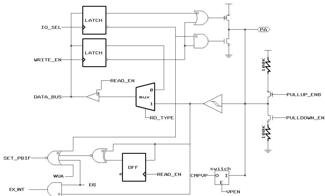
Figure 8 Block Diagram of PA3
