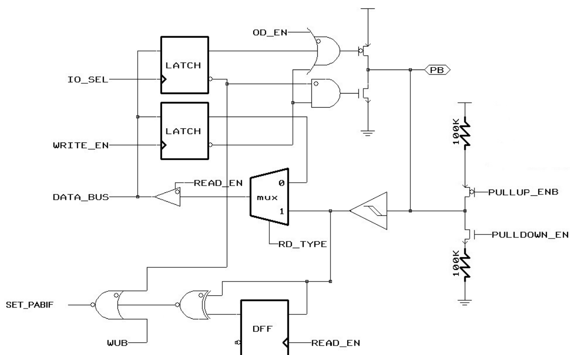
Figure 14 Block Diagram of PB2 & PB3
