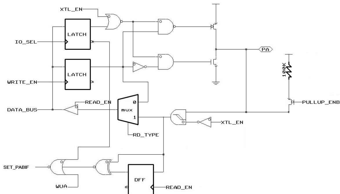
Figure 11 Block Diagram of PA6, PA7
