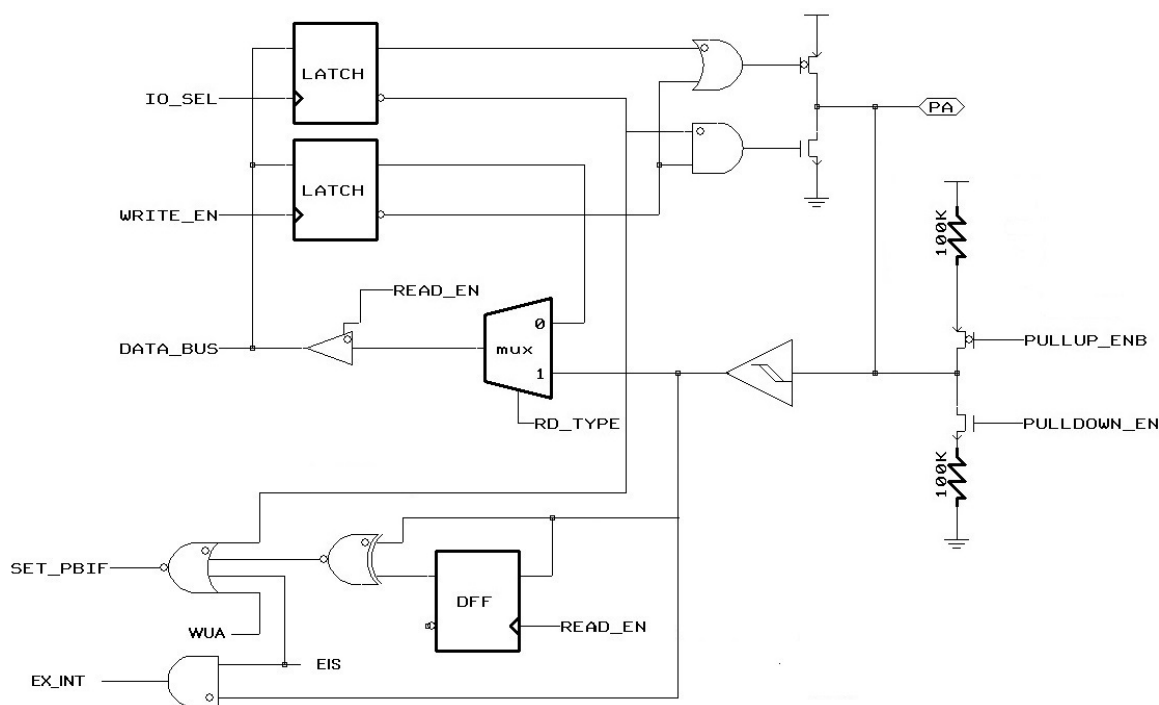
Figure 10 Block Diagram of PA5
