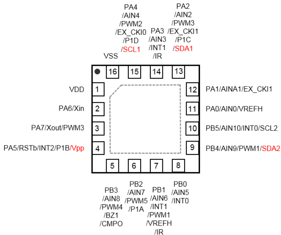
Figure 1 Package pin assignment
