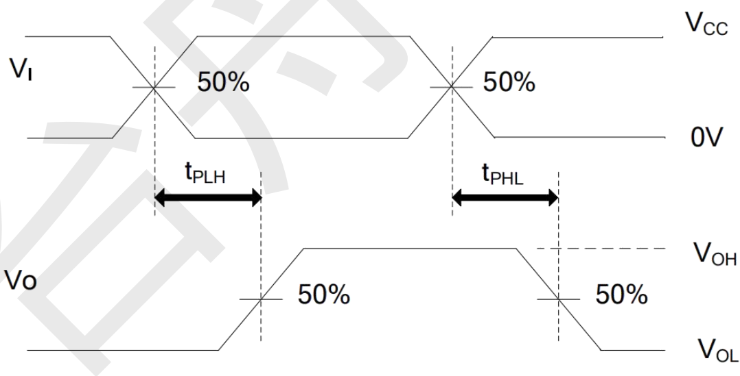
Propagation Delay Times
