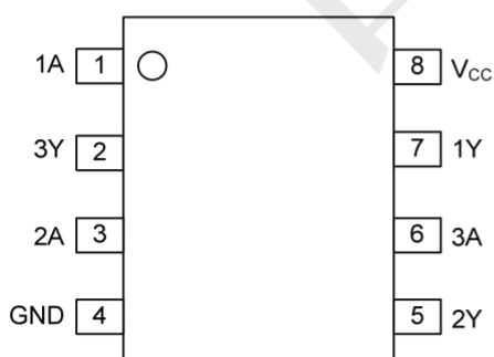
MSOP-8
