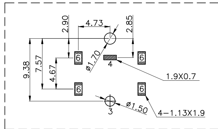
PCB.WELDING DRAWING (TOLERANCE:±0.05)
