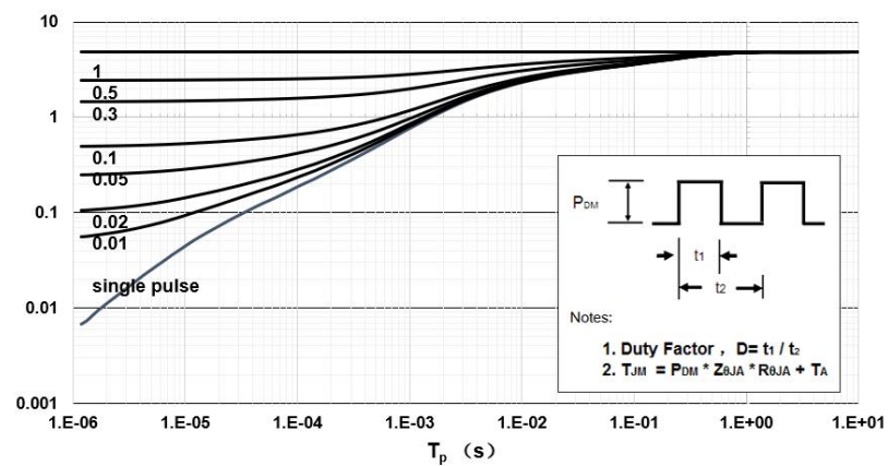
Figure 8. Max. transient thermal impedance
