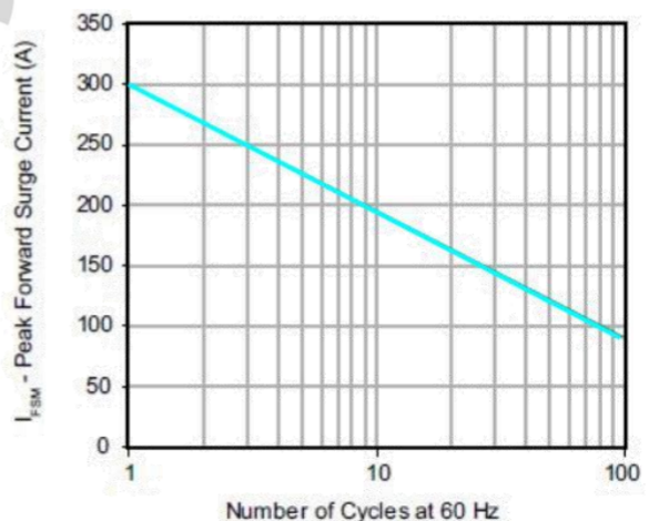
Maximum Non-Repetitive Forward Surge Current Uni-Directional Only
