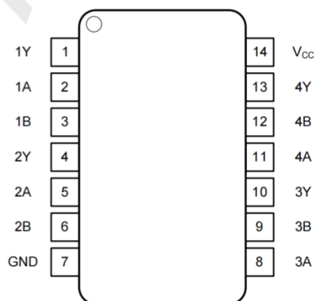
TSSOP-14
