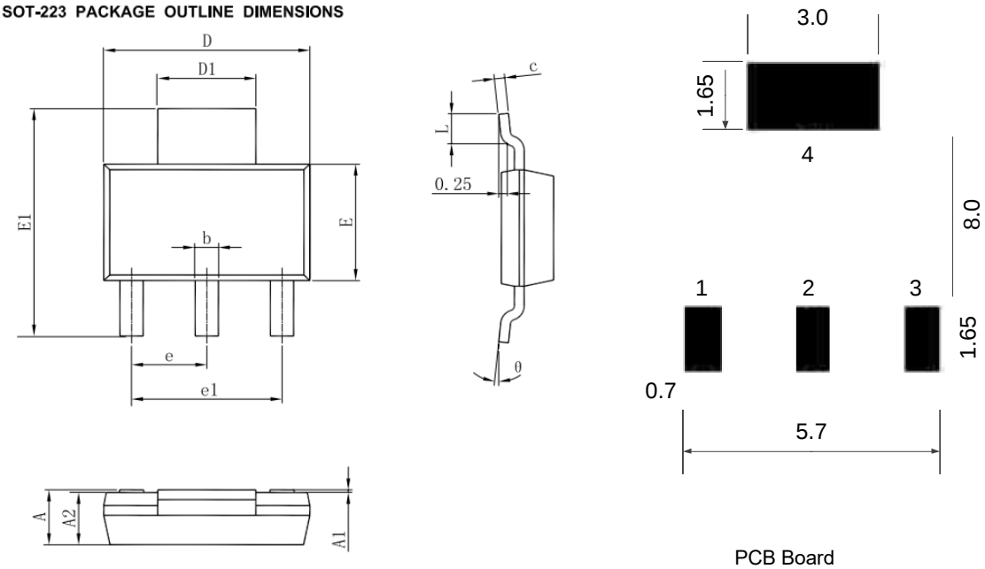
SOT-223 PACKAGE OUTLINE DIMENSIONS
