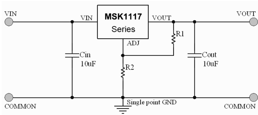
Application Circuit of MSK1117-ADJ
