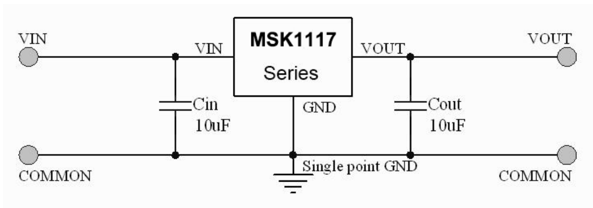
Application circuit of MSK1117 fixed version
