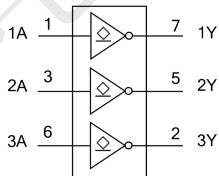
Logic symbol
