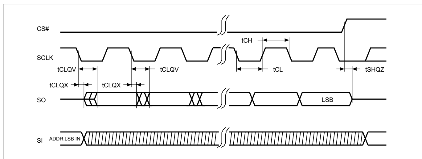
Figure 3. Output Timing
