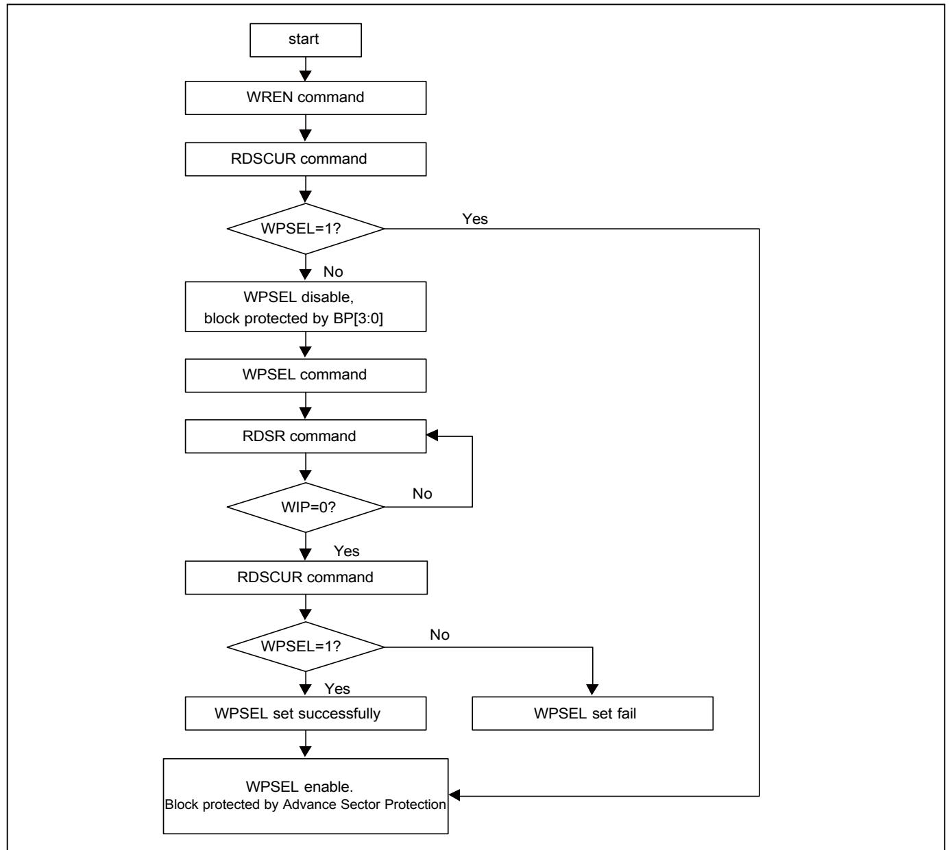
Figure 61. WPSEL Flow
