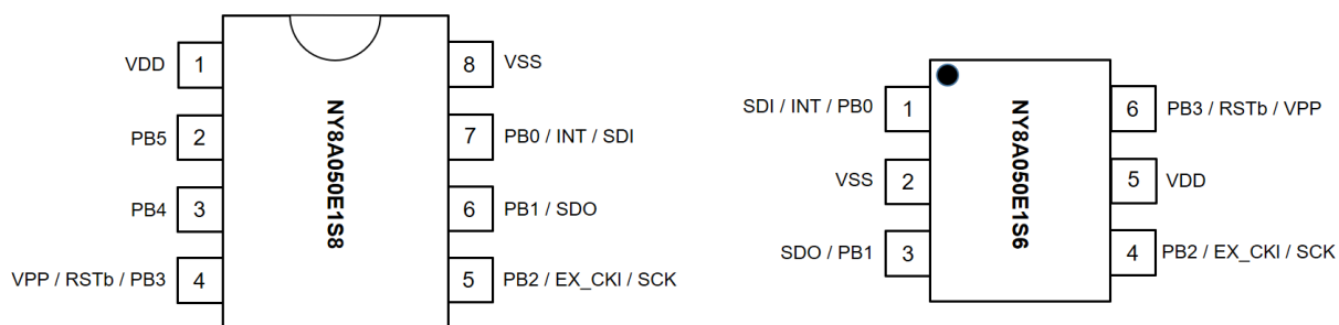
Figure 1 Package pin assignment
