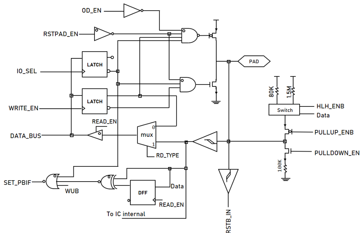
Figure 8 Block Diagram of PB3
