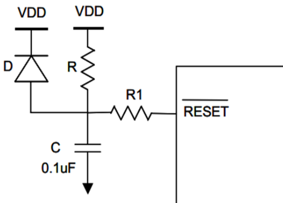
Figure 14 Block Diagram of Reset Application
