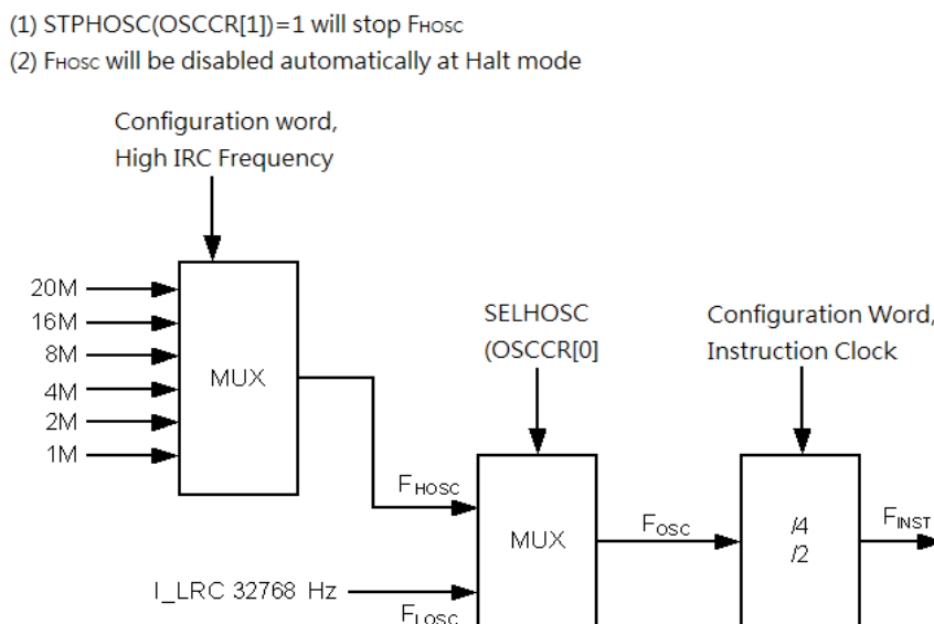
Figure 11 Oscillation Configuration of NY8A050E1
