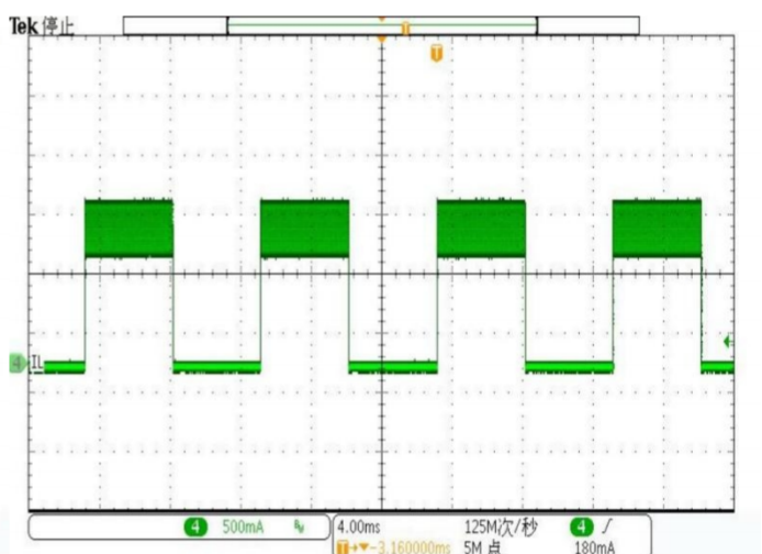
Fdim=100Hz Duty=50%
