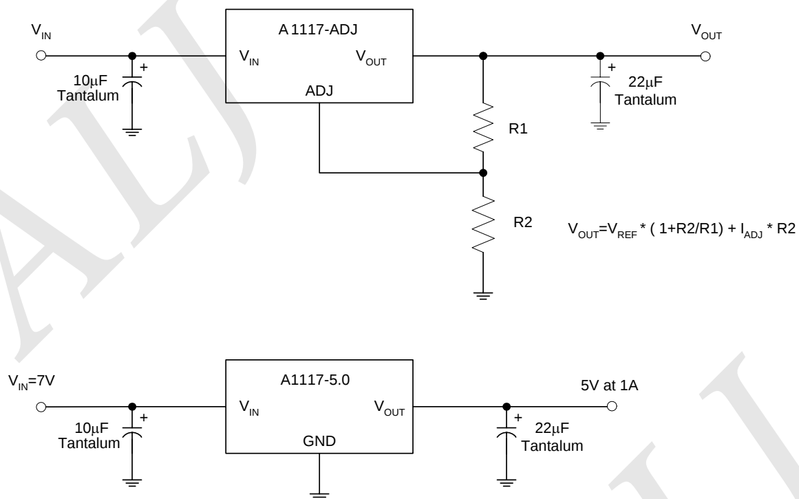
Figure 12. Typical Applications of AMS1117
