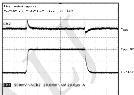
Figure 9. Line Transient Response
