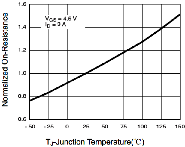
Figure 8 Drain-Source On-Resistance
