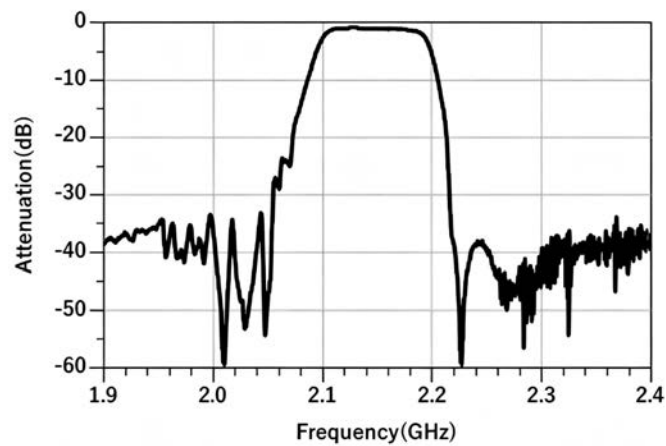
Narrowband
