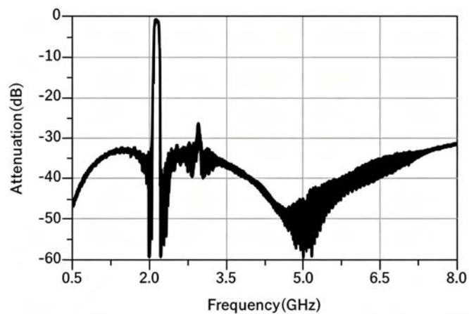
Wideband
