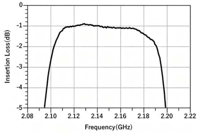
Passband
