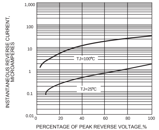
FIG. 4-TYPICAL REVERSE CHARACTERISTICS
