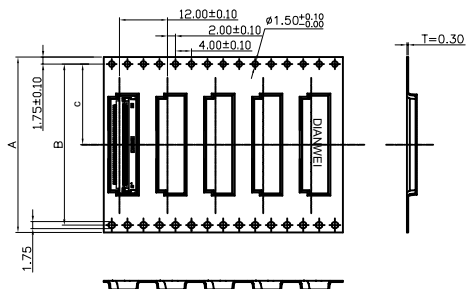
24~128PIN REEL
