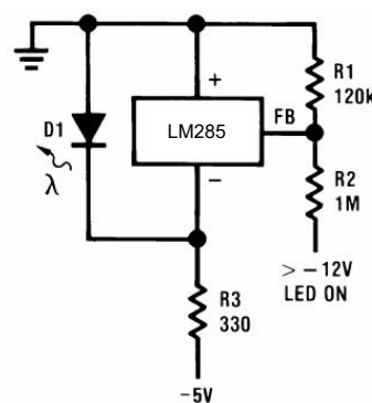
Figure 22. Voltage Level Detector
