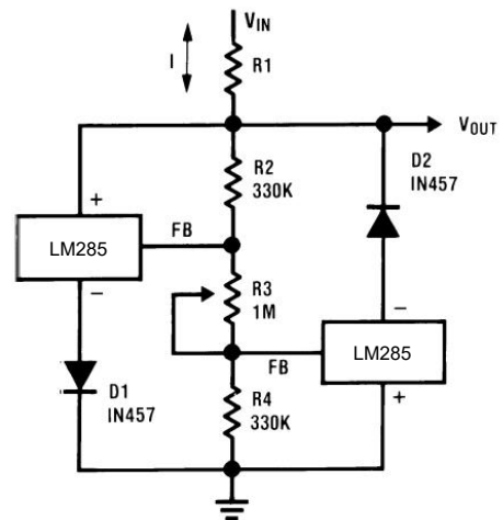
Figure 26. Bidirectional Adjustable Clamp \pm 2.4\text{V} to \pm 6\text{V}
