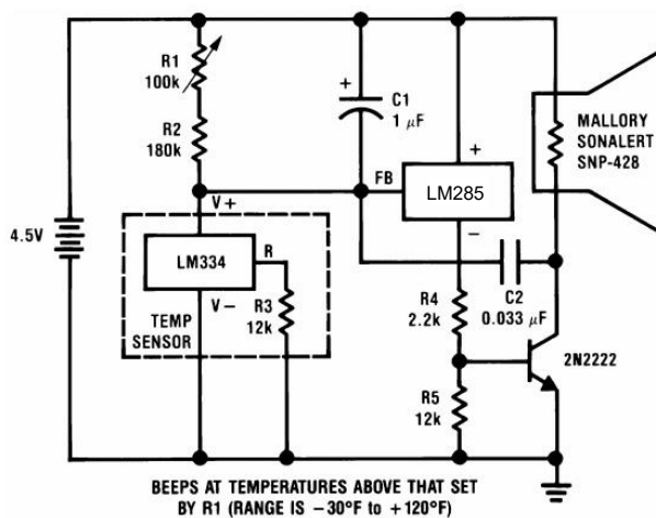
Figure 31. Freezer Alarm
