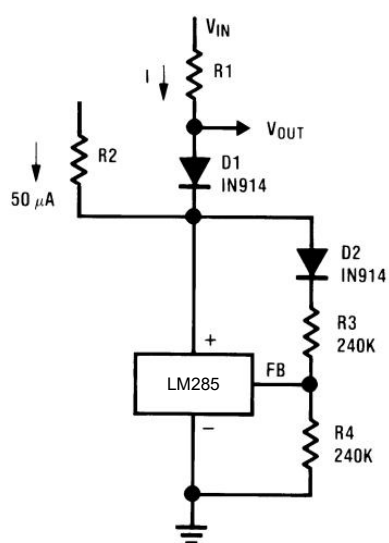
Figure 23. Fast Positive Clamp 2.4V + ΔVD1
