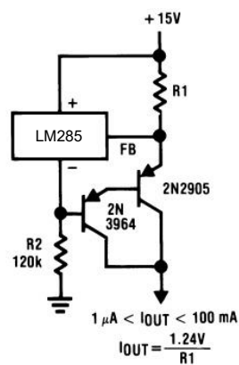
Figure 28. Current Source
