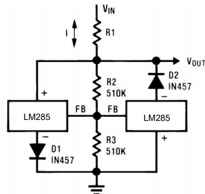
Figure 22. Voltage Level Detector
