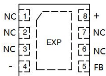
Figure 3. DFN Package Top View
