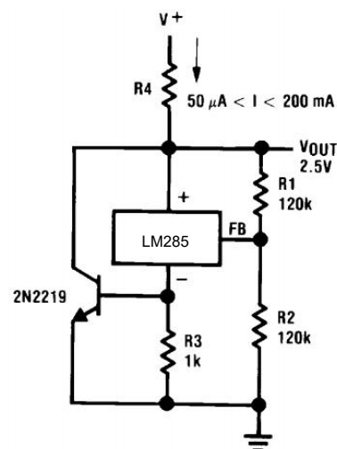
Figure 18. 200mA Shunt Regulator
