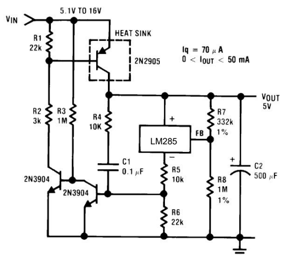
Figure 20. High Efficiency Low Power Regulator
