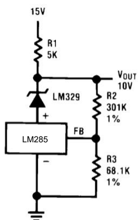
Figure 15. Precision 10V Reference
