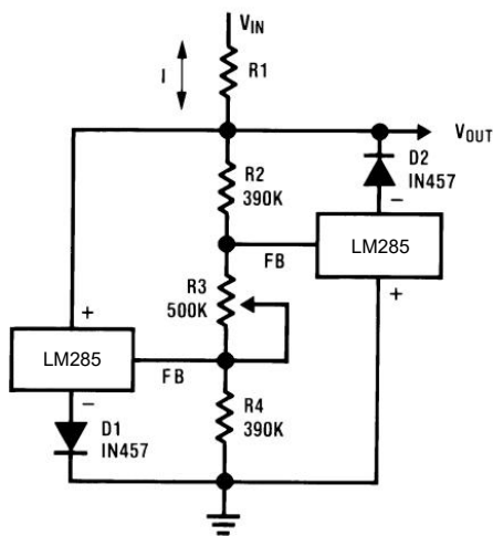
Figure 25. Bidirectional Adjustable Clamp \pm 1.8\text{V} to \pm 2.4\text{V}
