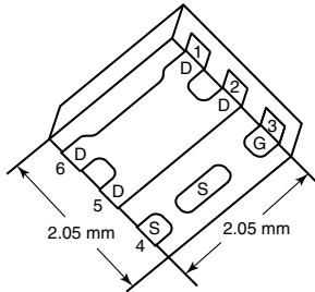
DFN2X2
