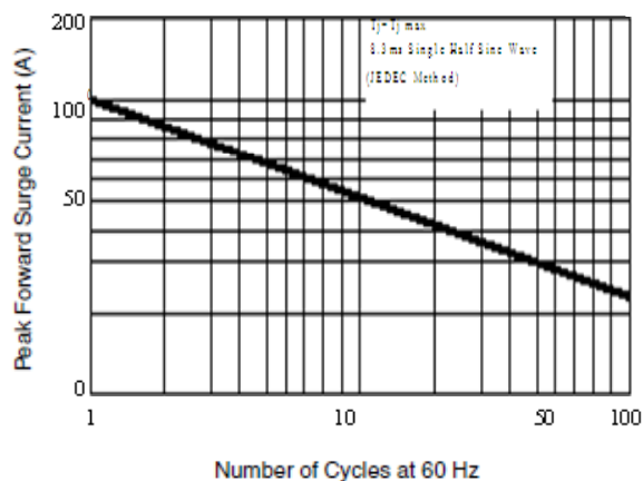
Figure 4. Max. Non-Repetitive Forward Surge Current Uni-Directional Only
