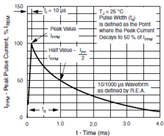
Figure 3. Pulse Waveform
