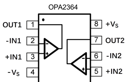
SOP-8/MSOP-8
