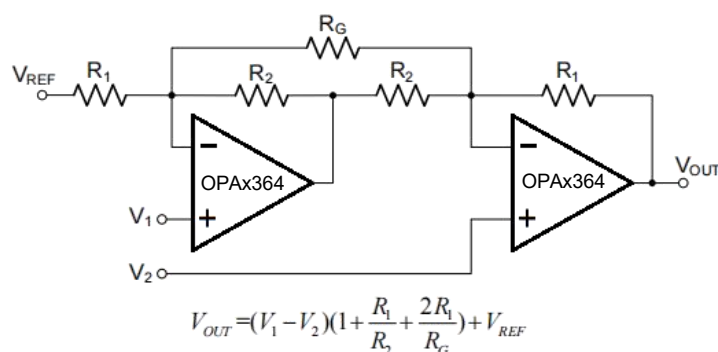
Figure 9. Instrumentation Amplifier
