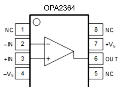
SOP-8/MSOP-8
